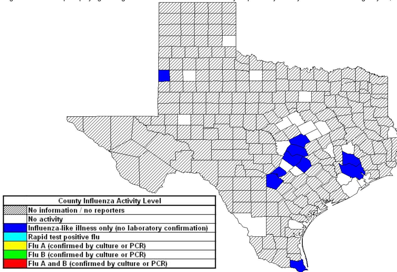
Figure 2: Texas Map Displaying the Highest Level of Influenza or ILI Activity Reported by County for the Week Ending July 25, 2020 (MMWR Week 30)
